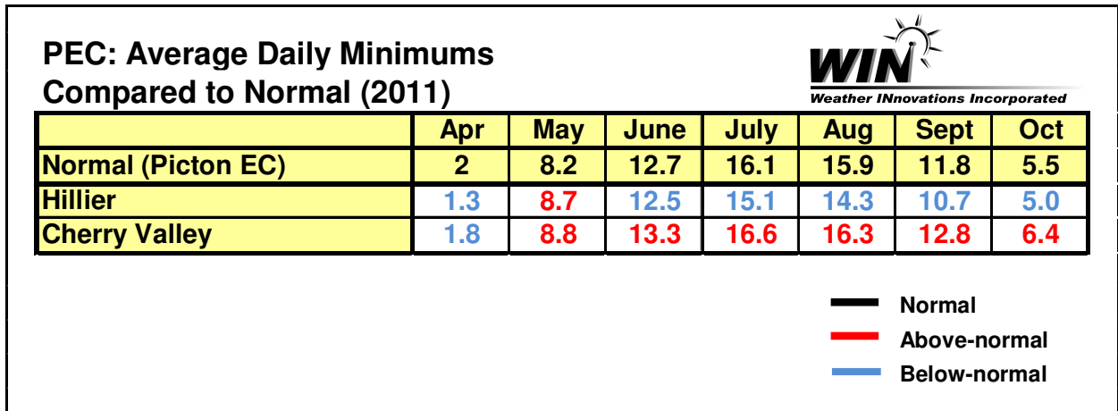
Figure 3: Minimum Temperatures
